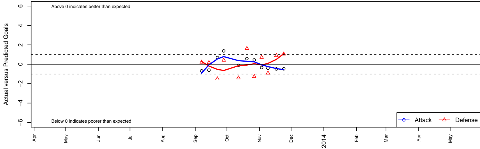
Pateadores Huntington Beach White B96 Dots are actual minus expected GF (blue circles) and GA (red triangles). Blue line is smoothed change in attack strength. Red is smoothed change in defense strength.
